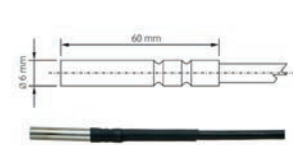
Pt1000TG68/E (-80°C to +200°C)
